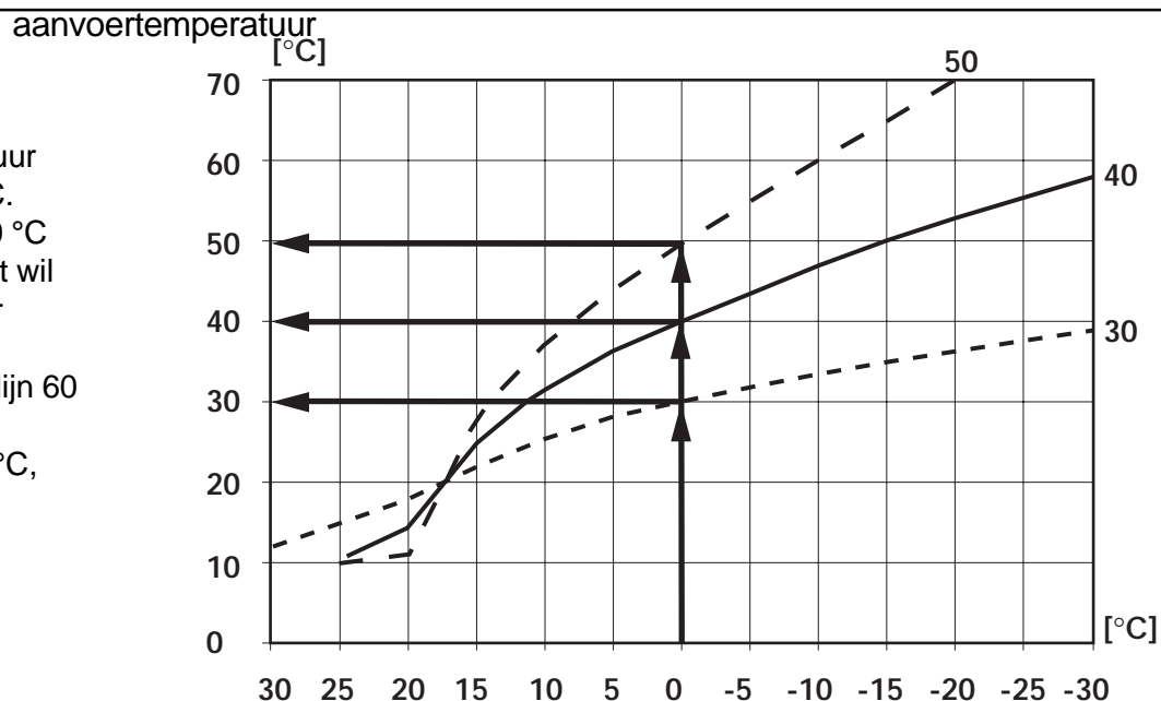
Fig. 20 Stooklijn
